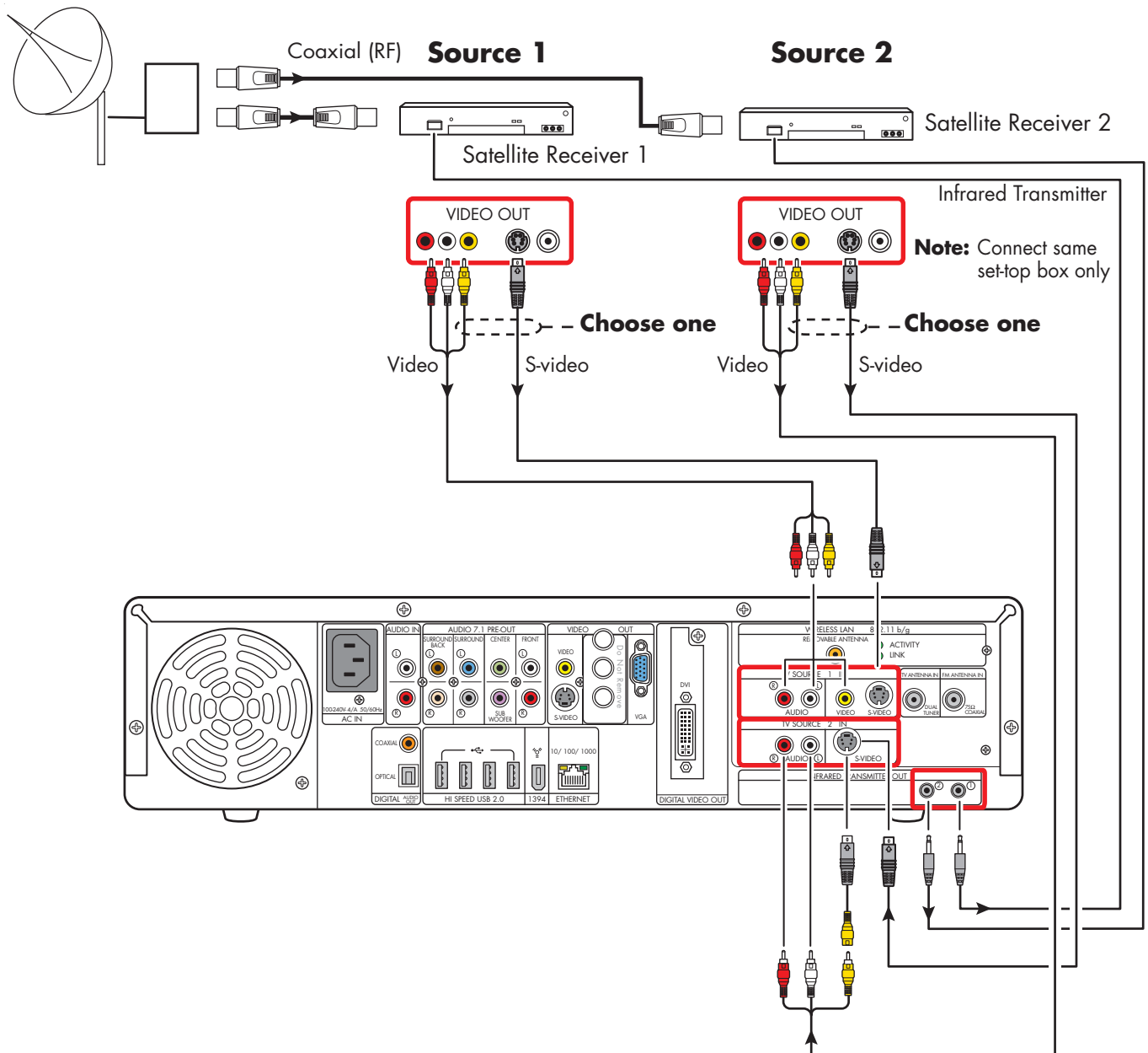
TV signal source – two satellite receivers (select models only)
